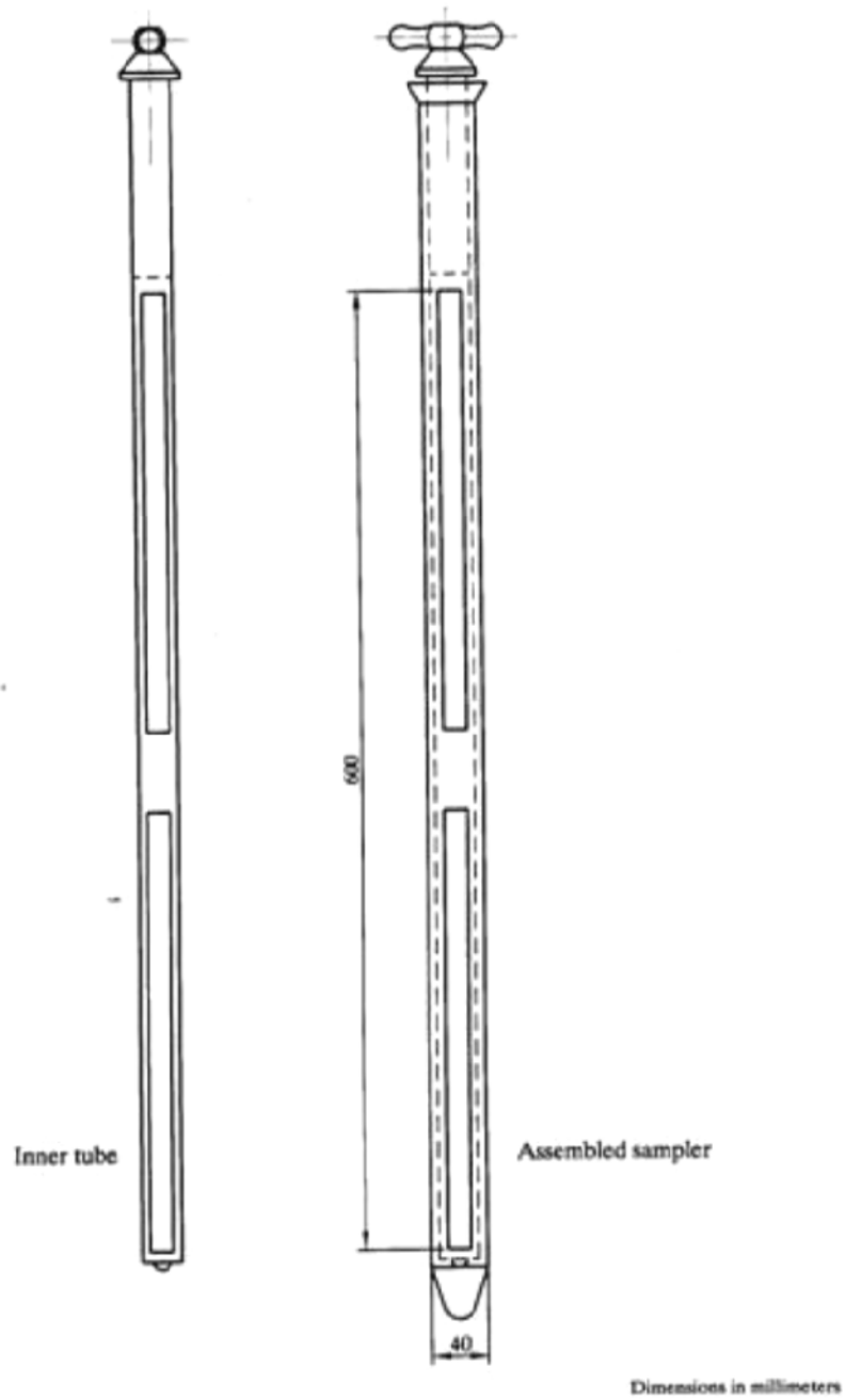
FIGURE 2 - Sampling Tube
