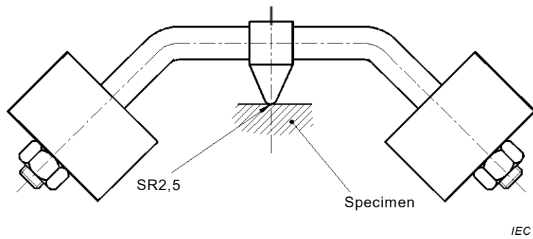
Figure 10 – Ball-pressure test apparatus
