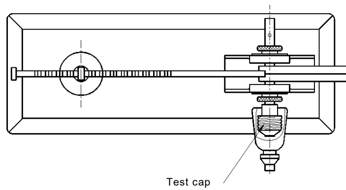
Figure 6 – Torque apparatus
