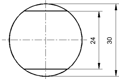
Figure 13a – Test cap A
