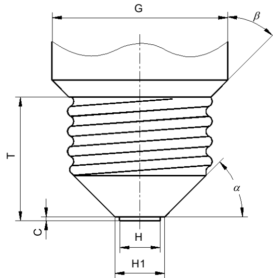
Figure 5b – Test cap E40
