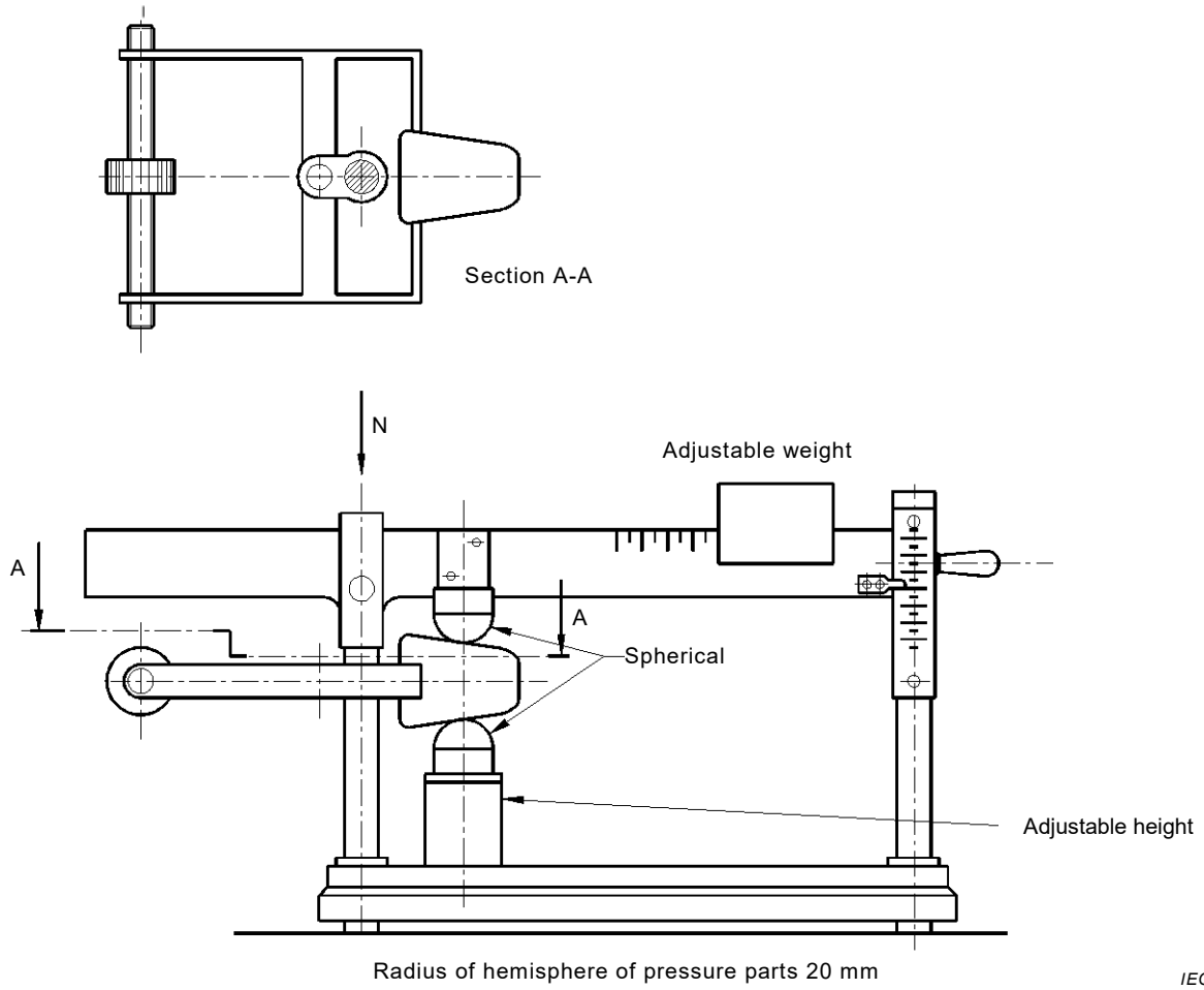
Figure 9 – Pressure apparatus
