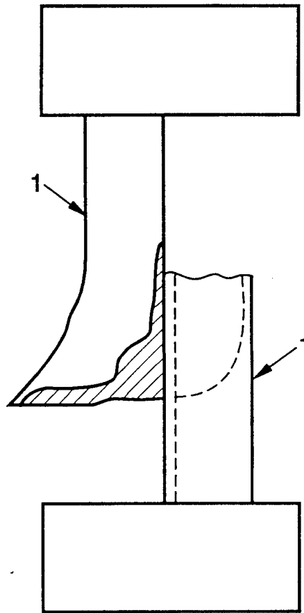
Figure D.2 - Clamping test specimens in the jaws
